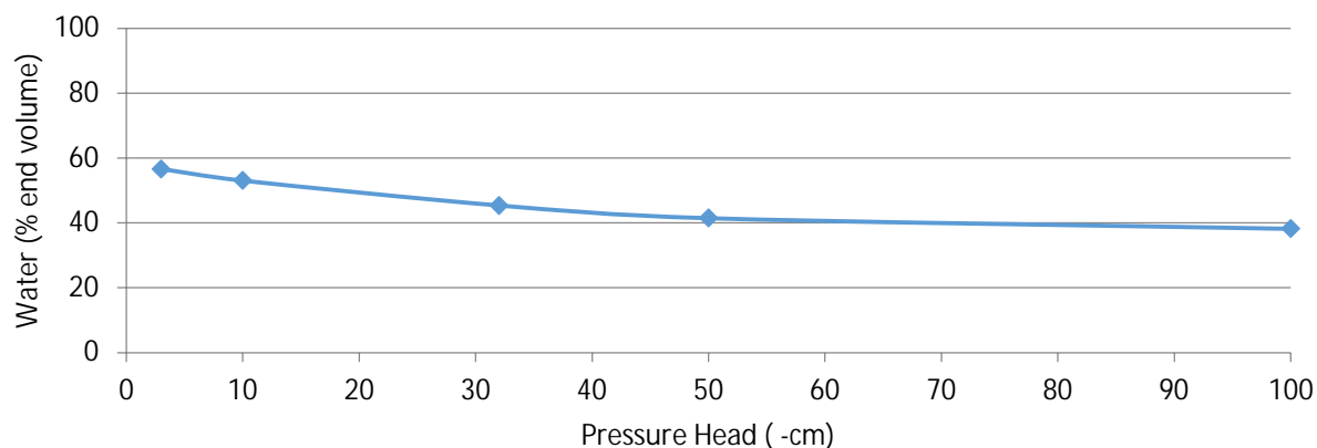
Waterretentioncurve
